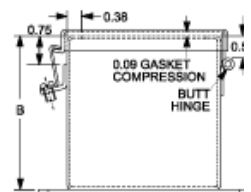
End View
