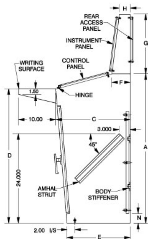
Section X-X
