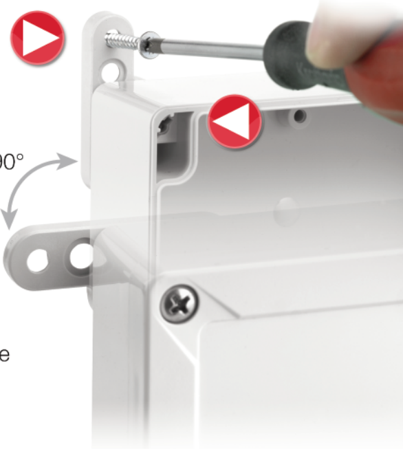
Enclosure mounts through corner holes or with optional mounting kit.
